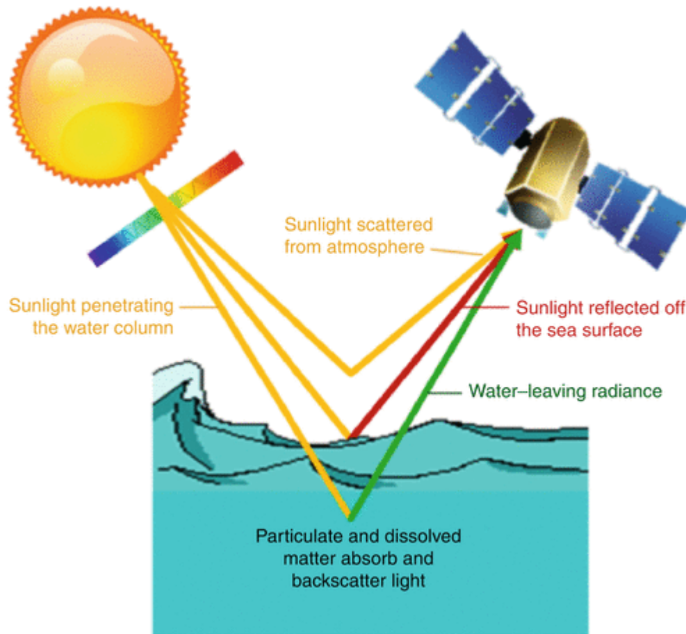
Remote Sensing of Ocean Color. Figure 4 Radiance measured by a satellite includes light scattered by the atmosphere and reflected off the sea surface (i.e., glint). In a process called "atmospheric correction," these signals are removed leaving the "water-leaving radiance" or the light that has penetrated the water column and been backscattered out to the satellite - a measure of ocean color
