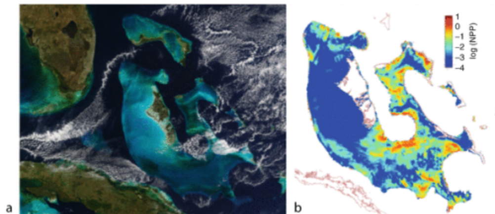
Remote Sensing of Ocean Color. Figure 7 The Great Bahama Bank is an example of optically shallow water where the seafloor color can be observed from space. (a) Pseudo-true color image from MODIS Aqua showing the bright Bahamas Banks with Florida, USA, to the West and Cuba to the Southwest. White wispy clouds can obscure the ocean color. (b) Net primary productivity ( \text{mgC m}^{-2} \text{d}^{-1} ) of seagrass and benthic algae estimated from ocean color imagery over the Great Bahama Bank [47]
