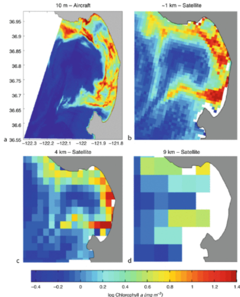
Remote Sensing of Ocean Color. Figure 3 Ocean color remote sensing imagery of Monterey Bay, California, illustrates different spatial resolutions available: (a) AVIRIS sensor flown on an aircraft, 10 m pixels [25]; (b) SeaWiFS satellite Level 2 data, 1 km pixels; (c) SeaWiFS satellite gridded to 4-km pixels; (d) SeaWiFS satellite Level 3 9-km standard product
