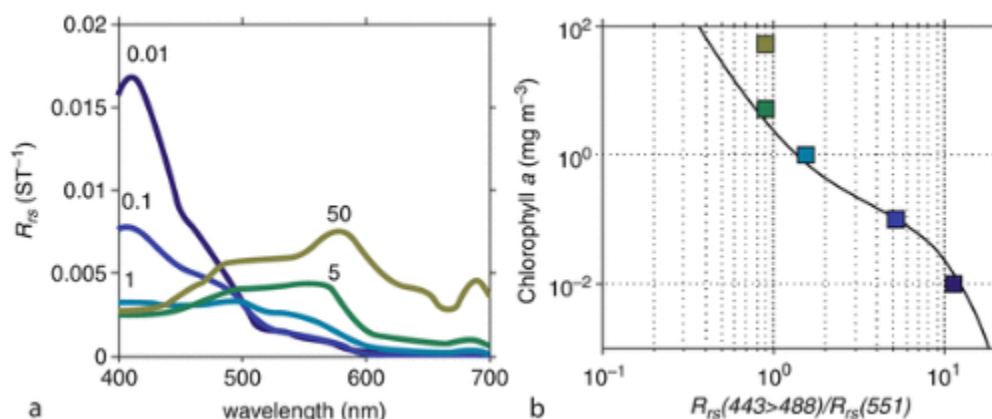
Remote Sensing of Ocean Color. Figure 5 (a) Remote sensing reflectance ( R_{rs} ) spectra modeled for different concentrations of chlorophyll a (Chl) from 0.01 to 50 \text{ mg m}^{-3} . The color of each line represents the modeled ocean color a human might observe following [61]. (b) The empirical OC3M model for deriving Chl from R_{rs} for the MODIS Aqua sensor. The model uses the "blue" channel with the highest R_{rs} value (443 or 488 nm) divided by the "green" channel at 551 nm. Each square represents the modeled Chl for the corresponding R_{rs} spectra in panel A and demonstrates how the model becomes less accurate at high Chl
