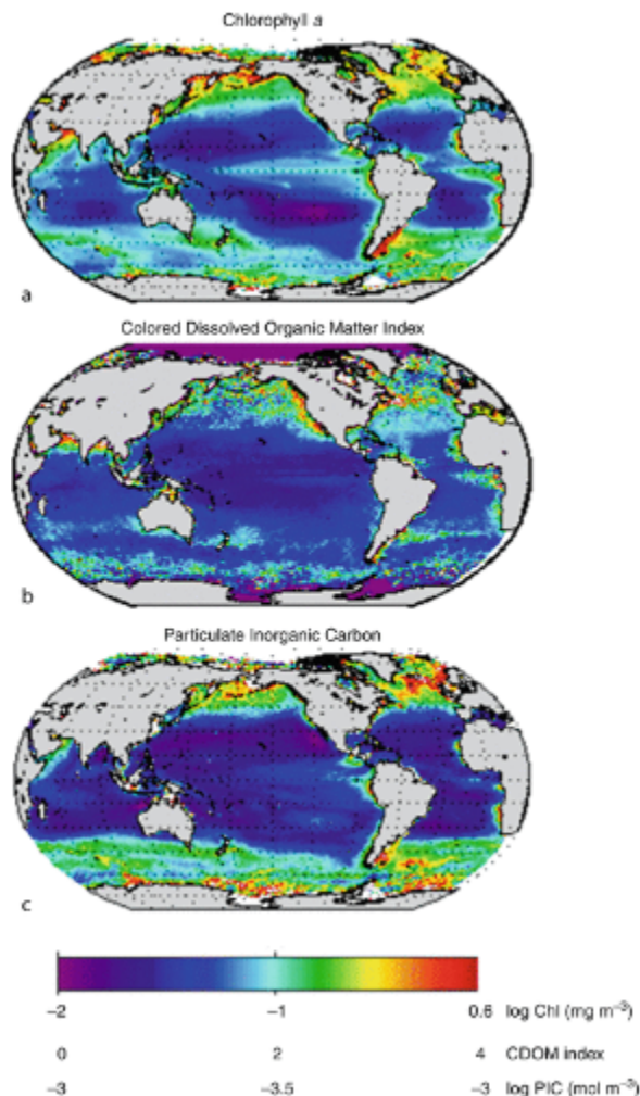
Remote Sensing of Ocean Color. Figure 8 Global climatologies or long-term averages of products derived from the Ocean Color SeaWiFS sensor from 1998–2011. (a) Chlorophyll a ( \text{mg m}^{-3} ); (b) colored dissolved organic matter (CDOM) index; (c) particulate inorganic carbon (PIC) ( \text{mol m}^{-3} )
