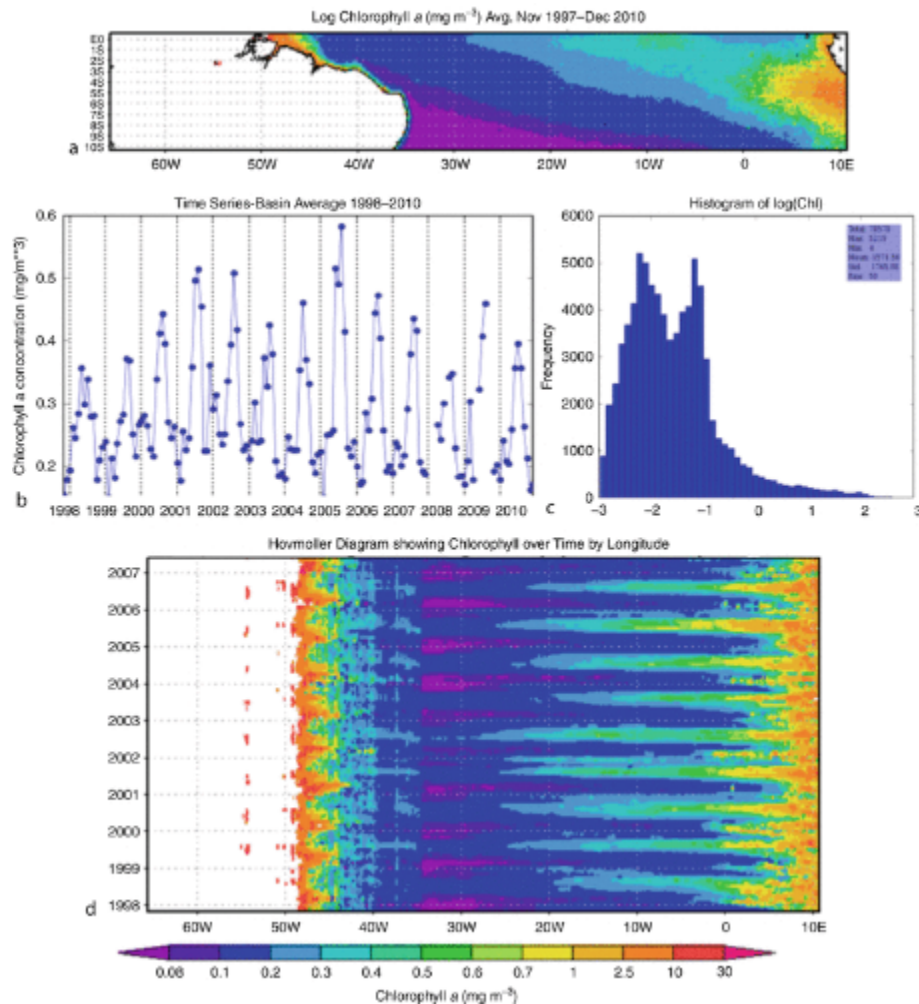
Remote Sensing of Ocean Color. Figure 6 Various times series analyses that can be conducted with standard Level 3 chlorophyll imagery including (a) Temporally averaged spatial distributions; (b) time series of interannual variability; (c) histograms showing the statistical distributions; (d) Hovmöller plots presenting both spatial (x-axis) and temporal (y-axis) variability. Such plots can be easily generated by the public with the Giovanni interface [59]
